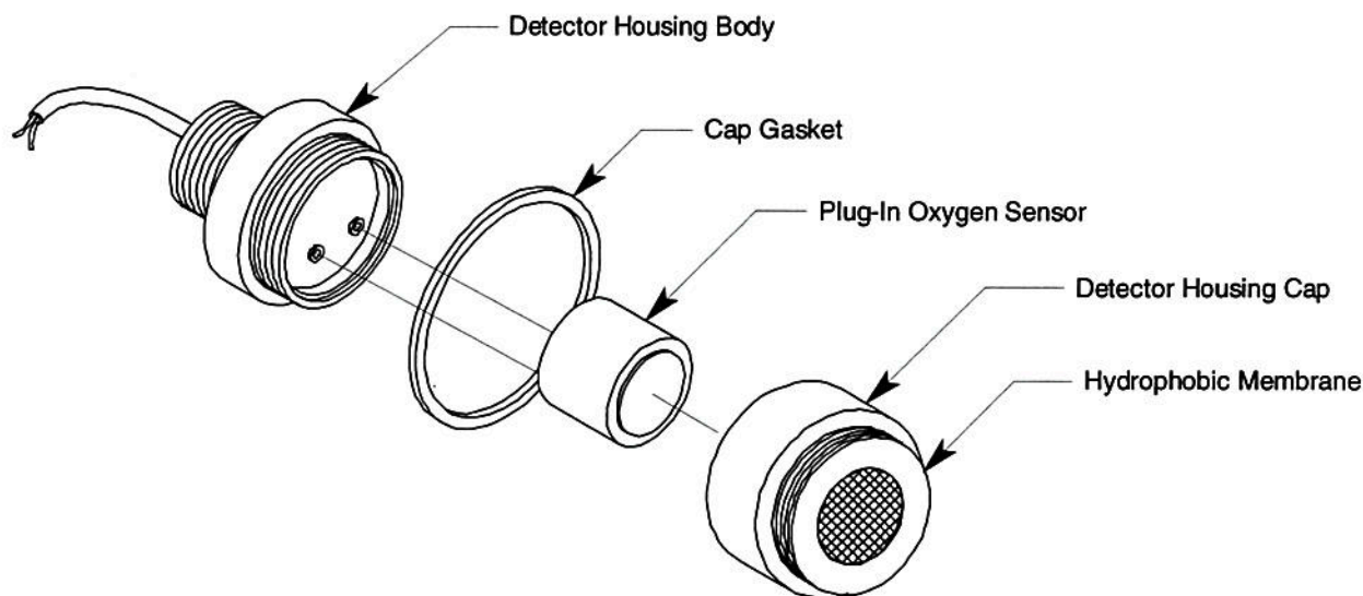
Figure 3: 65-2494RK Oxygen Detector, Non-Explosion Proof, Capillary Type
