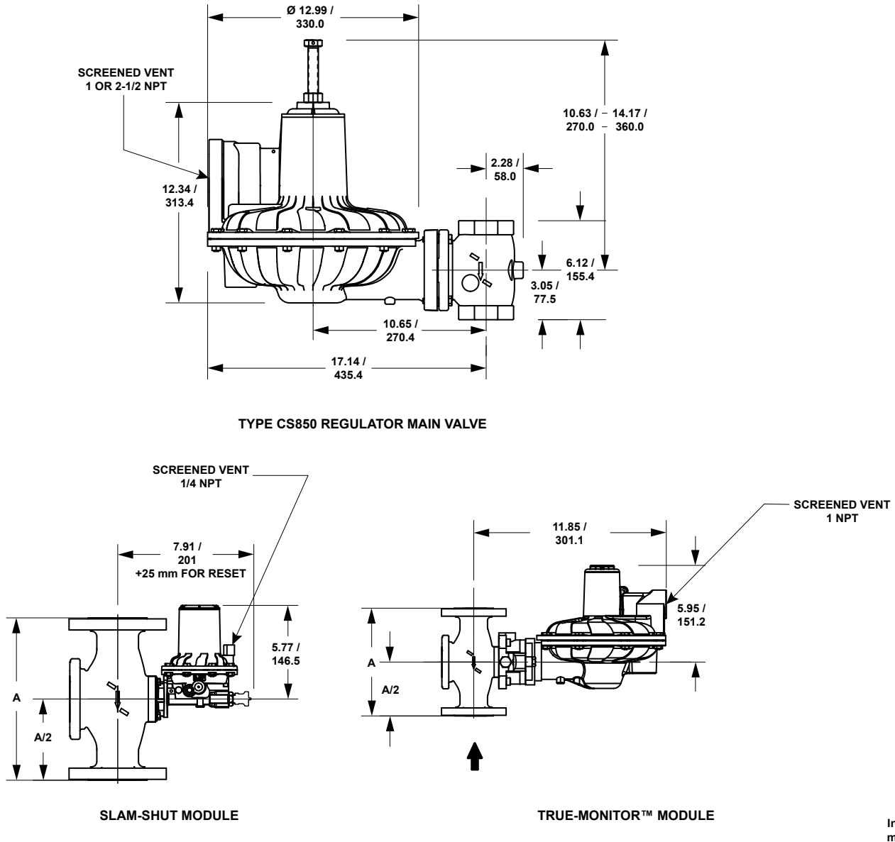
Figure 22. Dimensions (continued)
