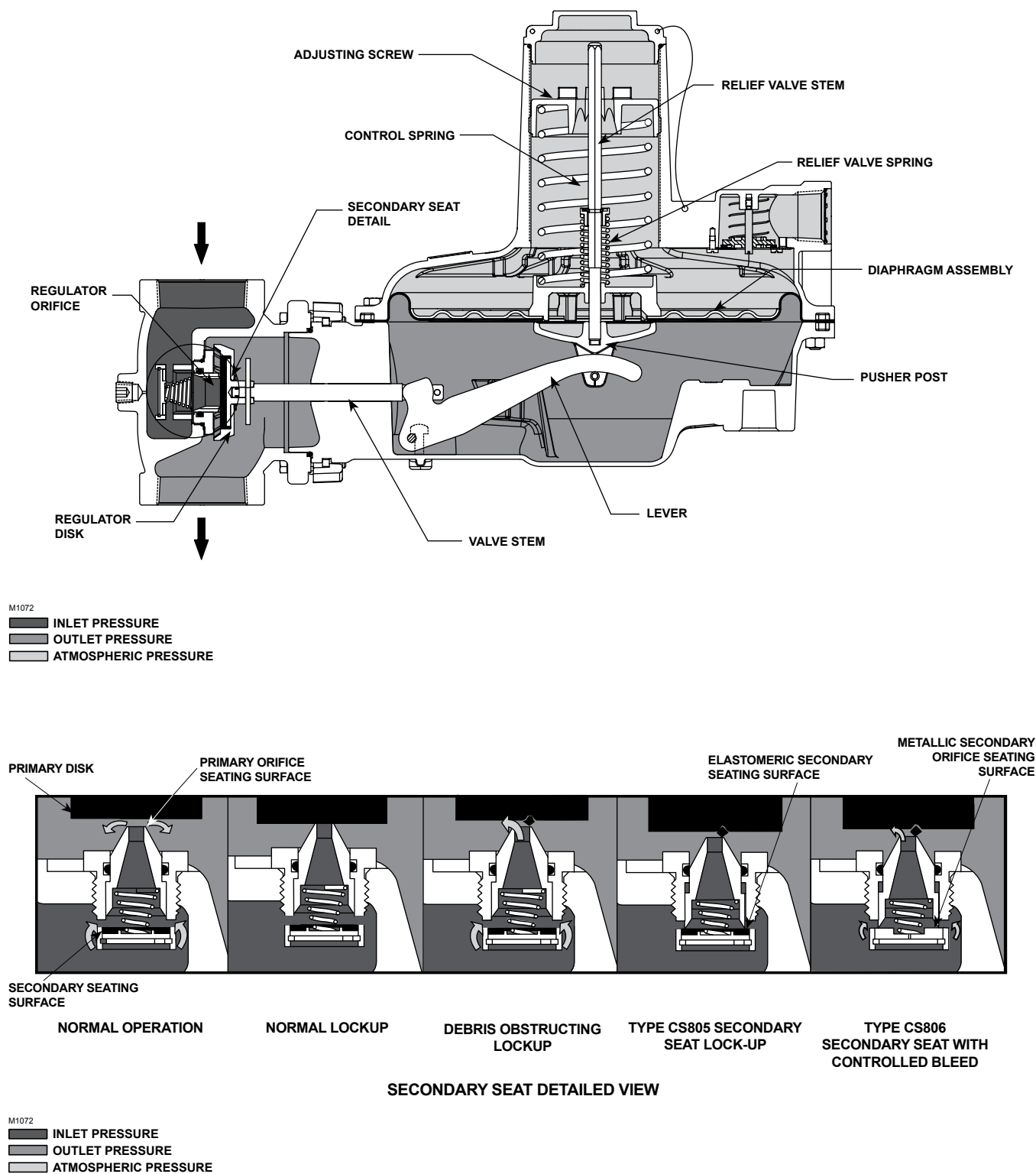
Figure 7. CS805 Series with Secondary Seat™ Protection
