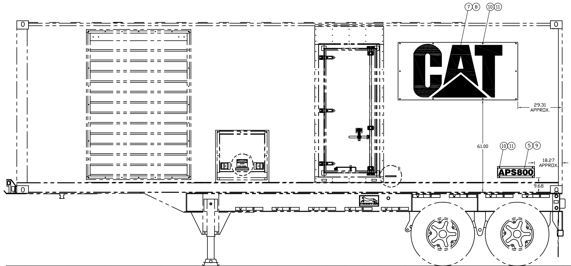
LEFT SIDE VIEW OF CONTAINER
