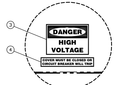
VIEW A AT E-6 SCALE 4=1
