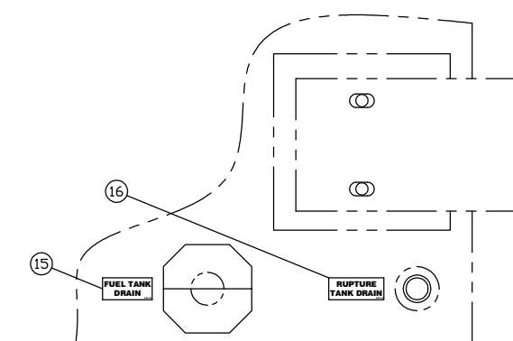
SECTION H-H AT E-4 SCALE 5=1
