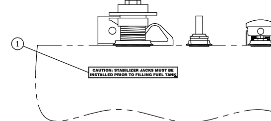
SECTION A-A AT B-7 SCALE 3=1
