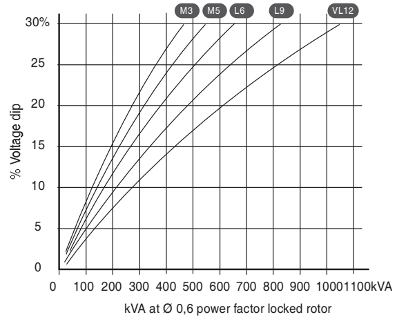
Motor starting (AREP or PMG excitation)
