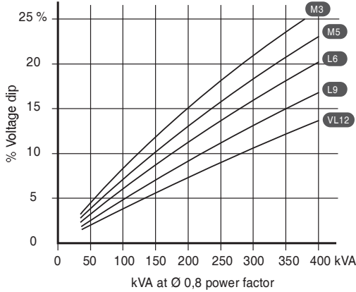
Load application (SHUNT excitation)
