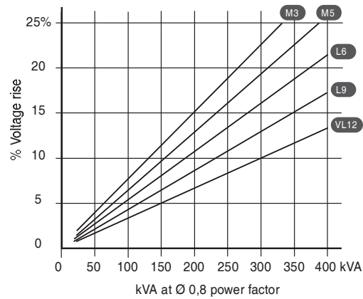
Load rejection (AREP or PMG excitation)
