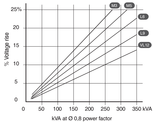
Load rejection (AREP or PMG excitation)
