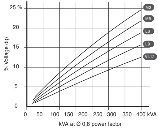
Load application (AREP or PMG excitation)
