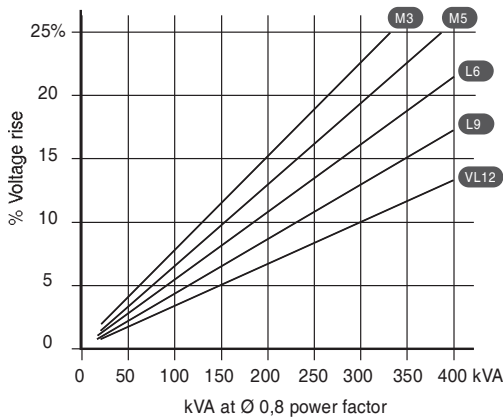
Load rejection (SHUNT excitation)
