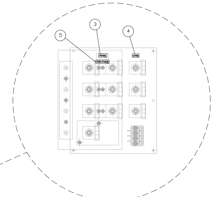
CHANGE OVER BOARD DETAIL
