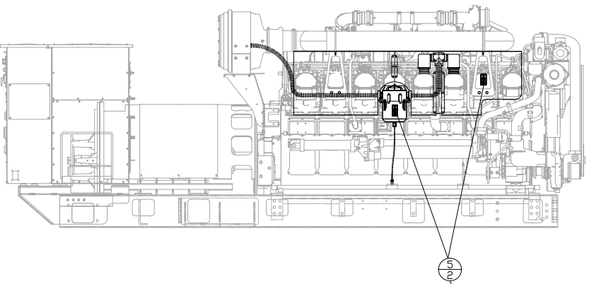
STREETSIDE POWER PACK VIEW
