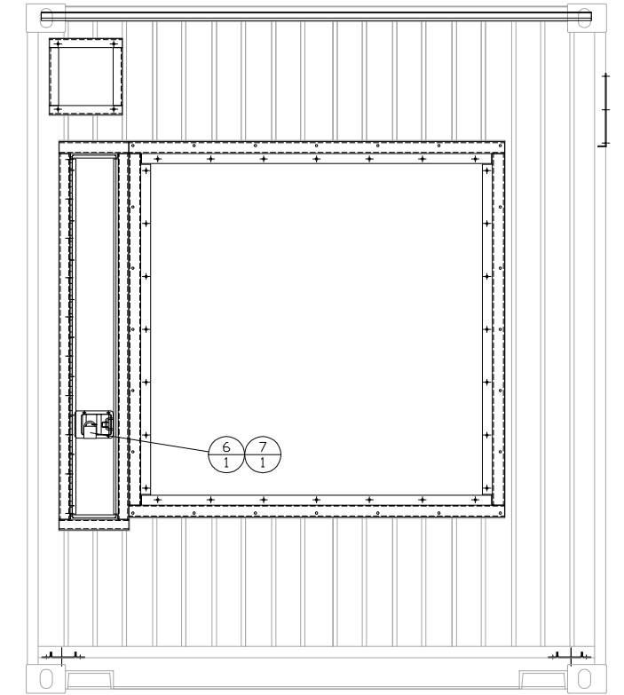
FRONT VIEW OIL MAKEUP DOOR CLOSED
