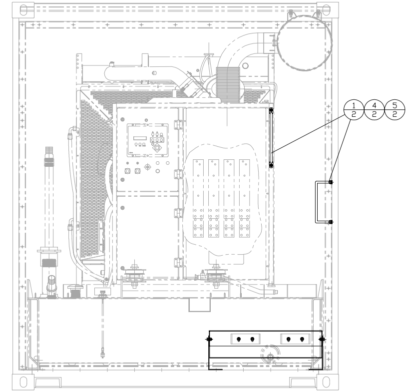
REAR VIEW BULKHEAD REMOVED
