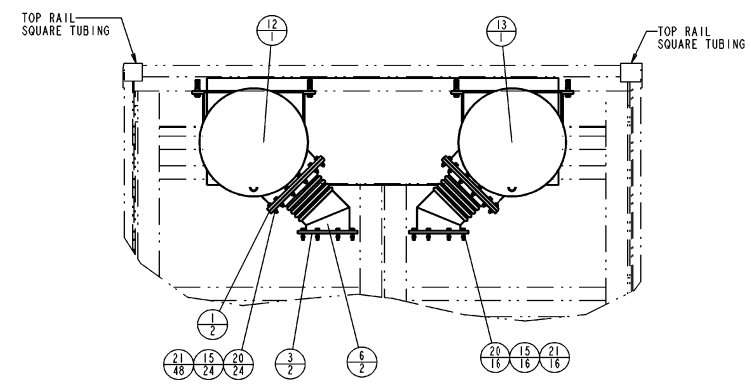
FRONT VIEW (FRONT WALL AND INSULATION NOT SHOWN FOR CLARITY)
