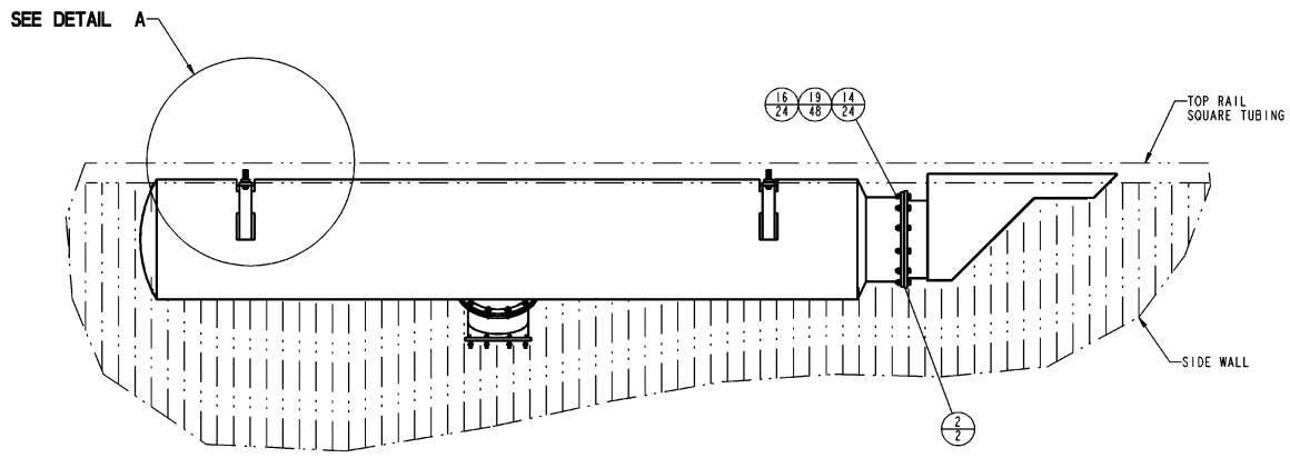
ROADSIDE VIEW (ROADSIDE WALL AND INSULATION NOT SHOWN FOR CLARITY)
