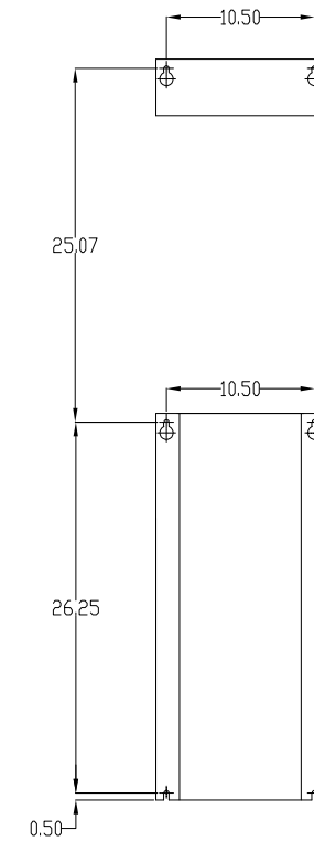
DRILLING DETAIL
