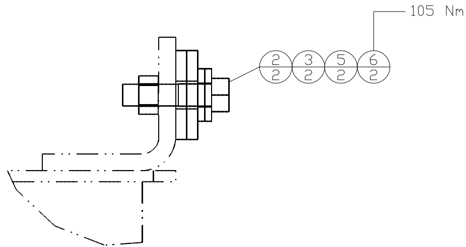
DETAIL B
