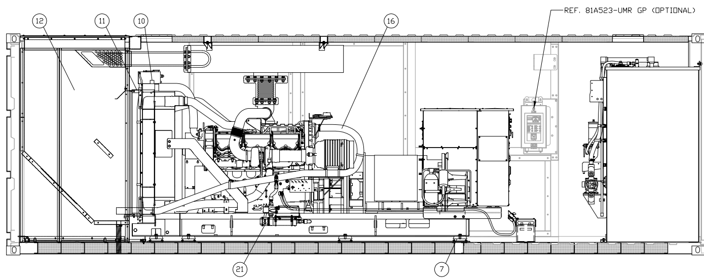
CURB SIDE VIEW (WALL REMOVED)
