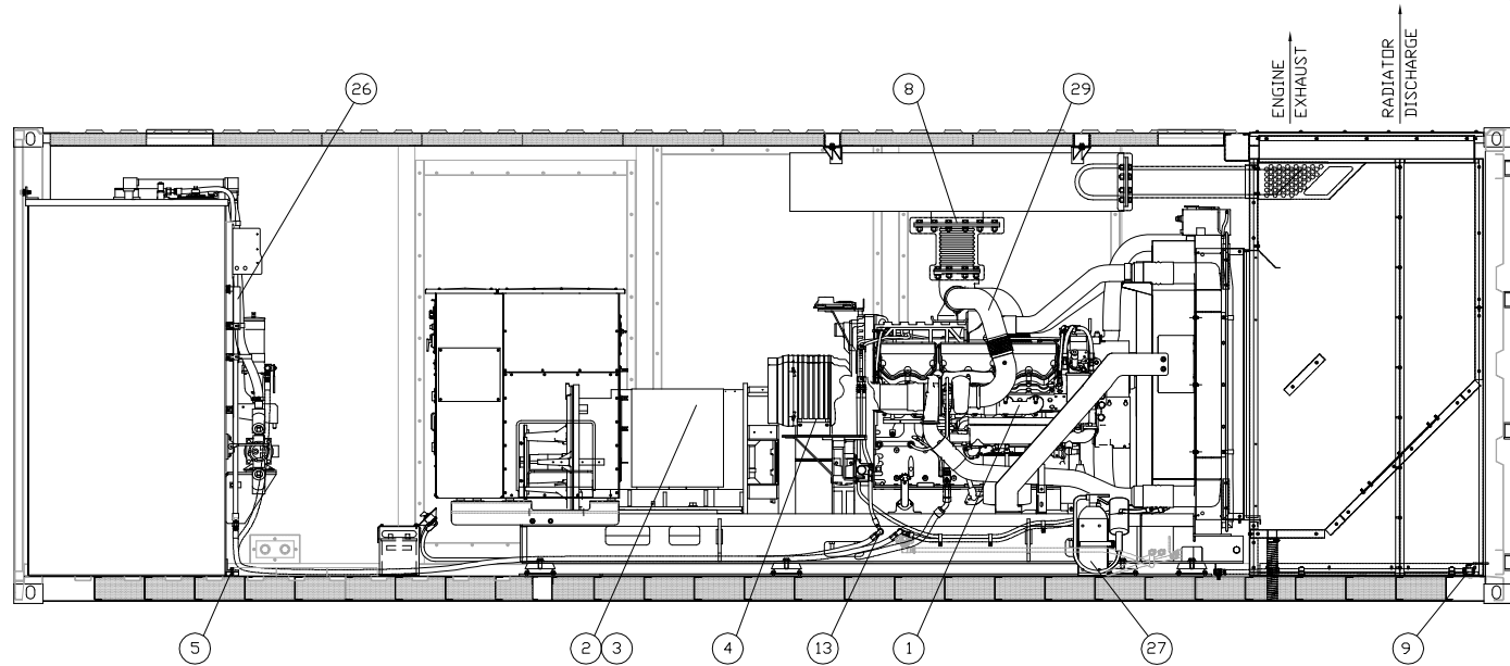
STREET SIDE VIEW (WALL REMOVED)
