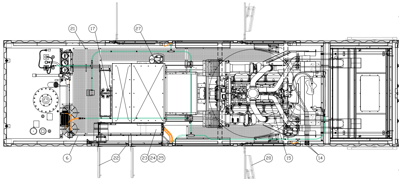
TOP VIEW (ROOF REMOVED)
