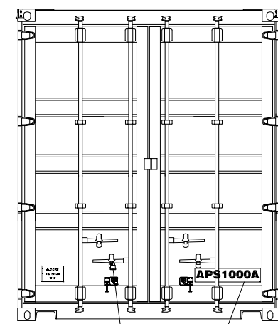
REAR VIEW (DOORS CLOSED)
