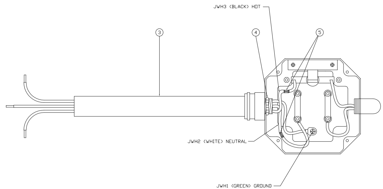
VIEW BB SCALE 1=10
