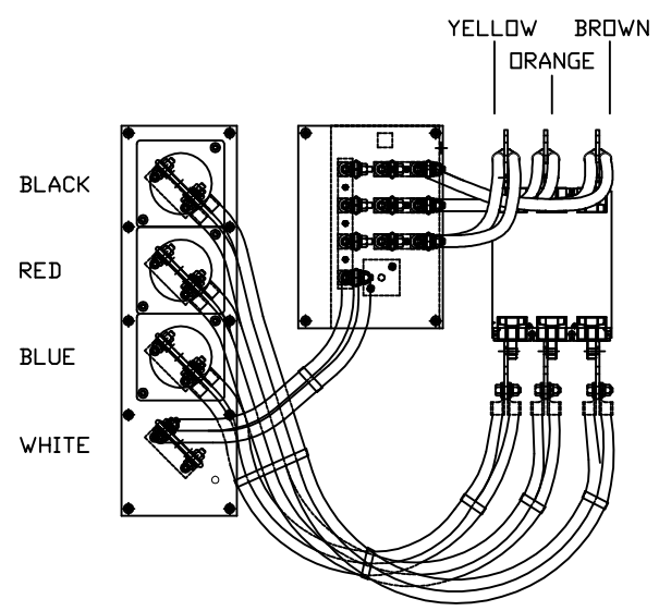
CABLE LAYOUT
