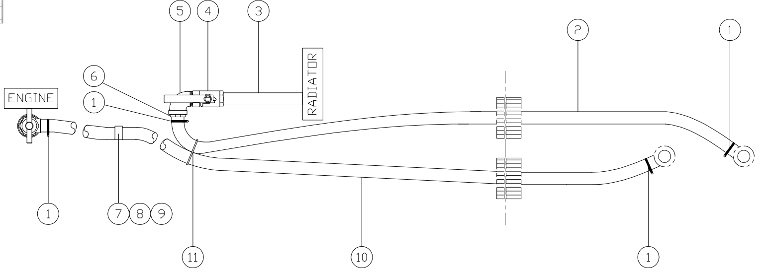
HOSE ASSEMBLY-SIDE VIEW SCALE 3=1
