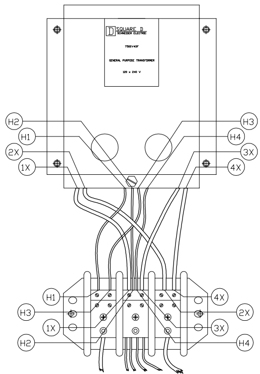
DETAIL A TRANSFORMER CONN. SCALE 4:1
