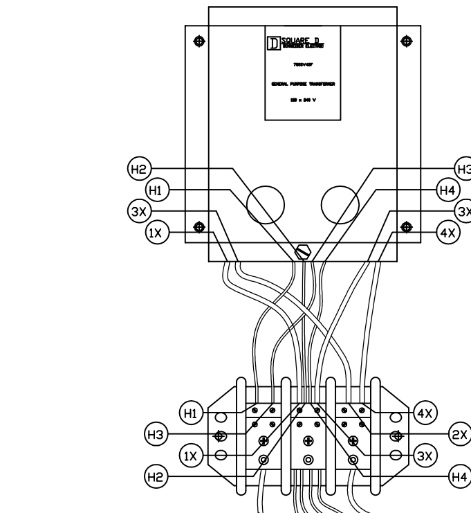
DETAIL A TRANSFORMER CONN. SCALE 4:1
