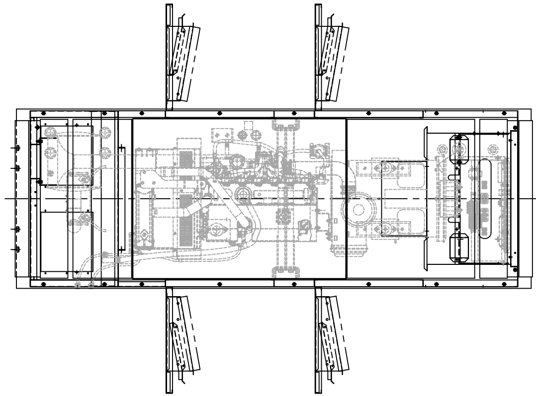
TOP VIEW ROOF REMOVED
