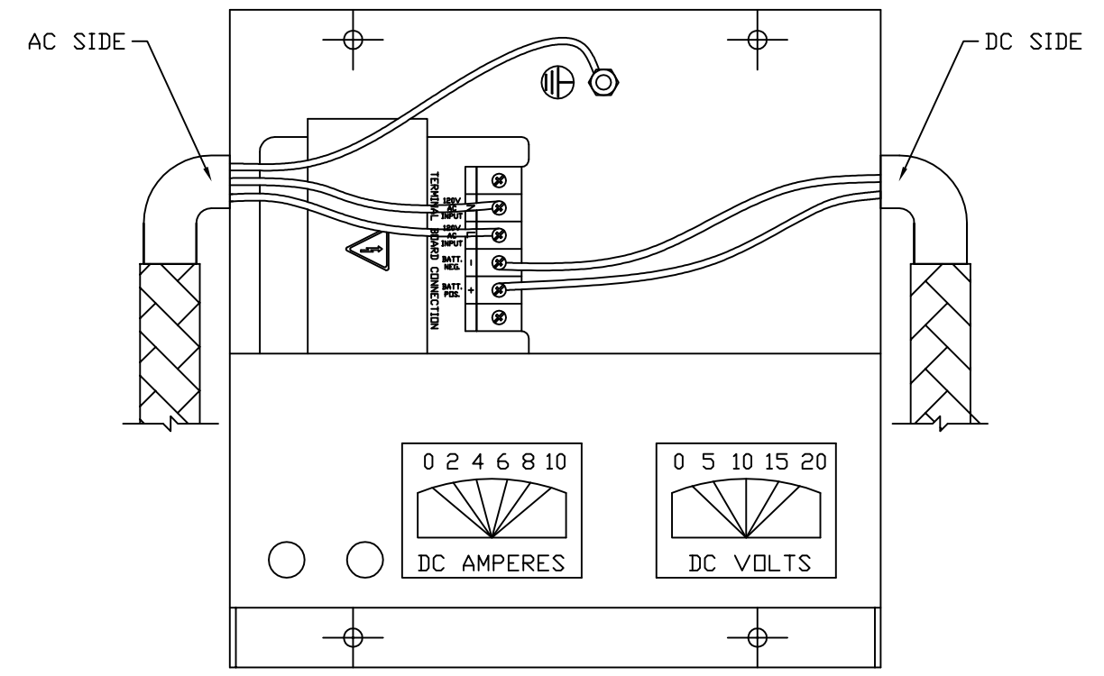
FRONT VIEW (BATTERY CHARGER) SCALE 5:1
