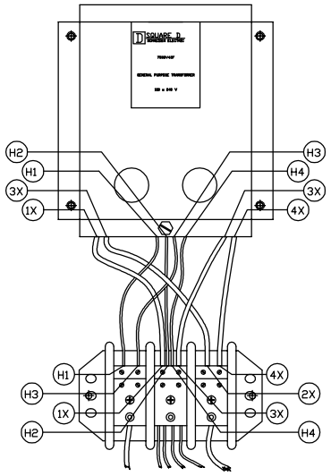
DETAIL A TRANSFORMER CONN. SCALE 4:1
