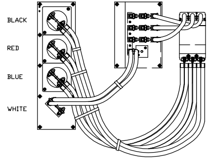
CABLE LAYOUT
