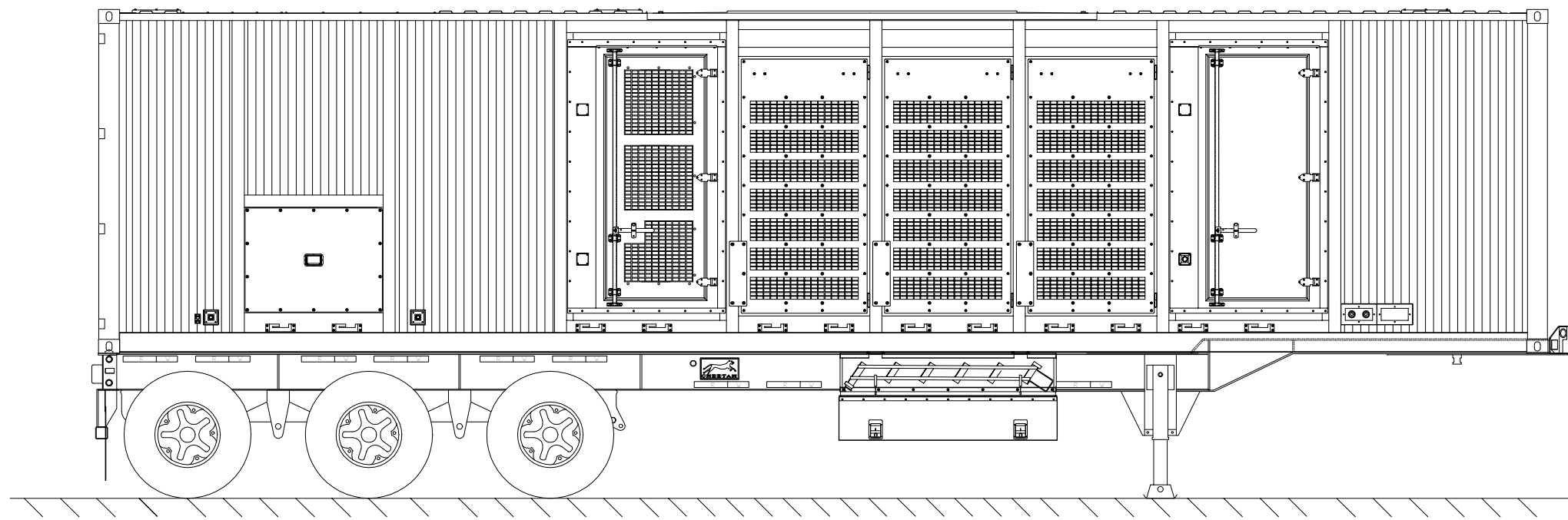
CURBSIDE VIEW
