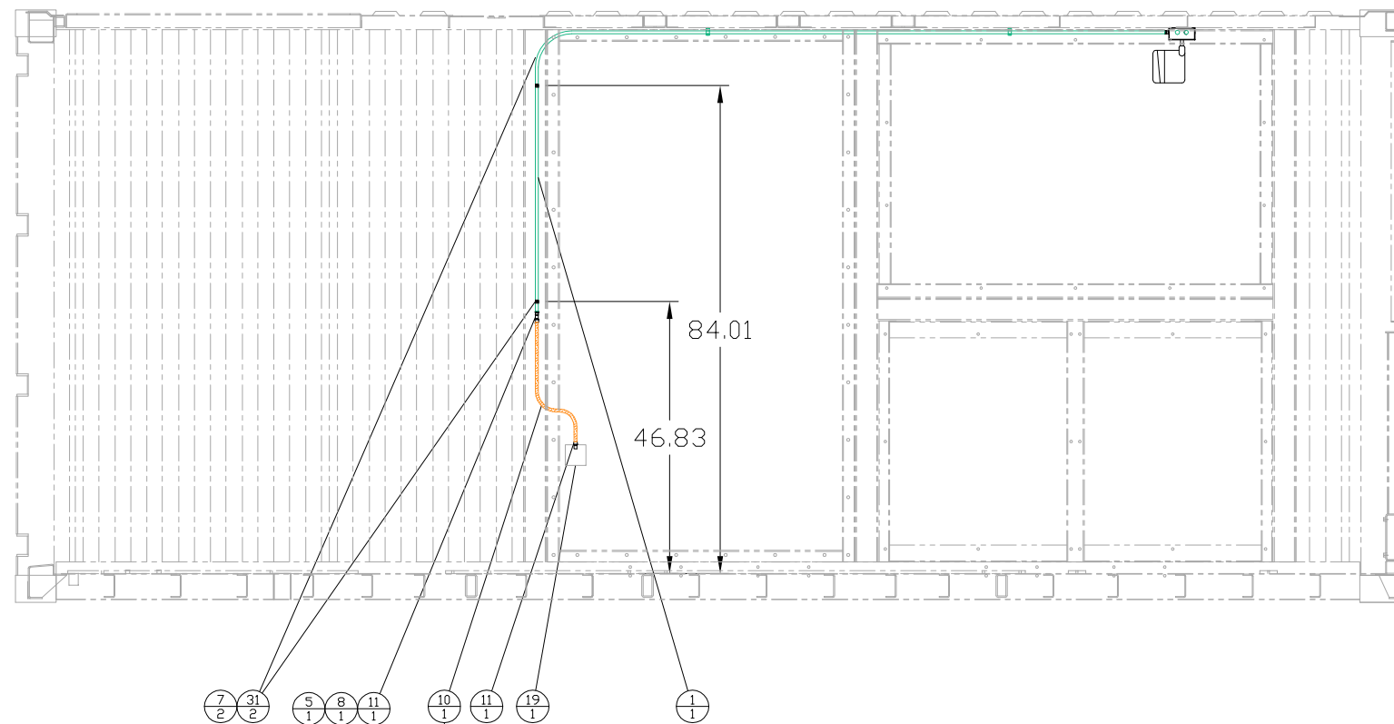
STREET SIDE VIEW SECTION A-A
